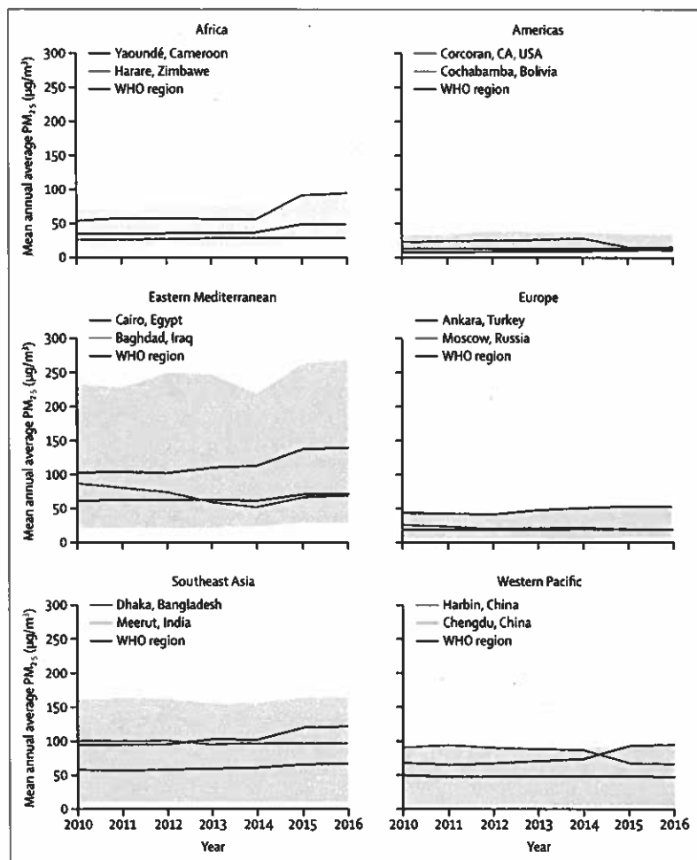
Figure 17: Mean of annual average PM_{2.5} concentrations over the period 2010–16 for Sustainable Healthy Urban Environments cities by WHO region, estimated using digital marketing qualification. WHO regions are represented by blue lines. Also shown are the range for all cities (light blue shaded area) and cities with the largest decrease (green lines) and increase (red dotted lines) over the period based on linear trends. PM_{2.5} = atmospheric particulate matter with a diameter of less than 2.5 \mu m .
